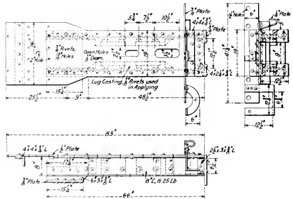
Rolled Steel Draft Arm for the E. J. & E.
